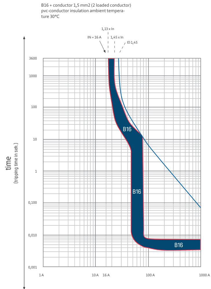
Fig. 12: Characteristic curve for planning example 1
