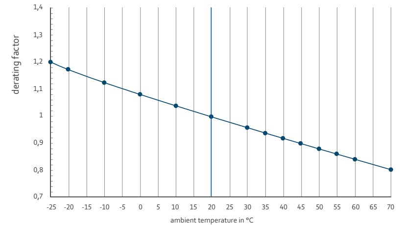
Fig. 23: Derating for K, Z characteristic
