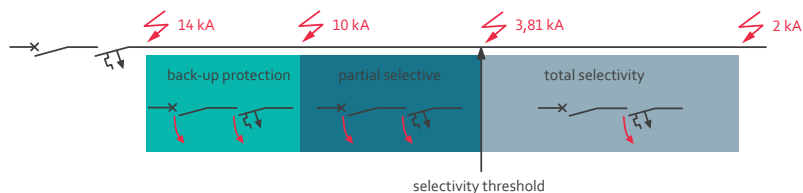
Fig. 18: Partial selectivity
