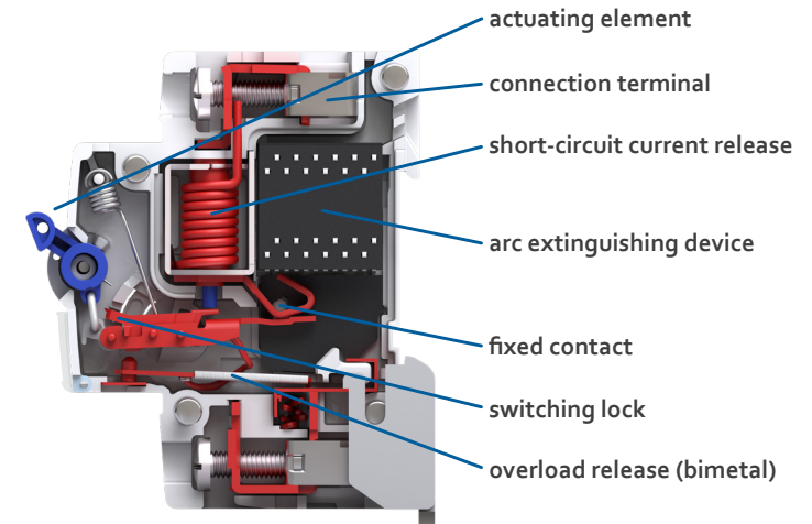
Fig. 1: Typical structure of a miniature circuit-breaker
