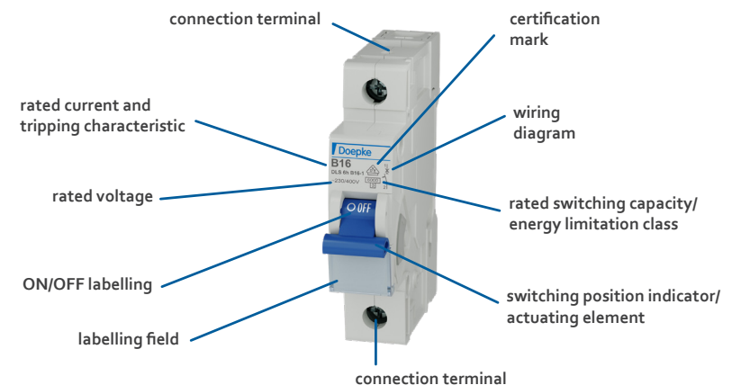
Fig. 3: Overview and labelling
