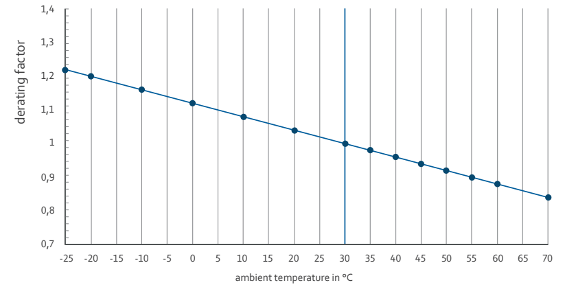
Fig. 22: Derating for B, C, D characteristic
