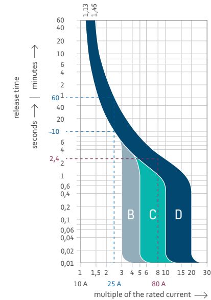
Fig. 7: Tripping curves for B, C, D characteristic
