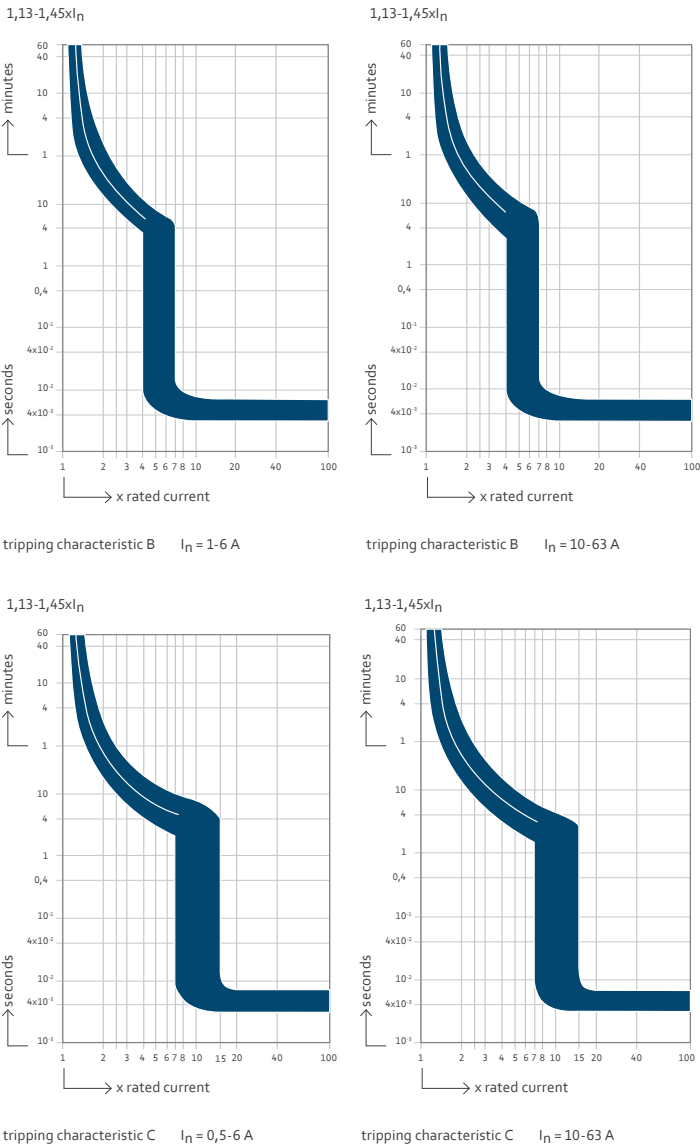
Fig. 28: DLS 6 hdc tripping characteristic curves
