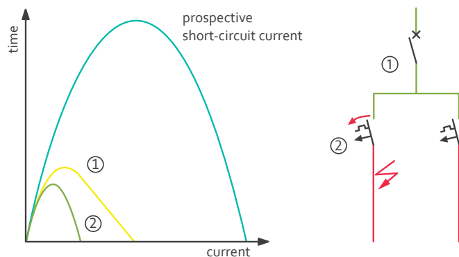
Fig. 19: Backup protection
