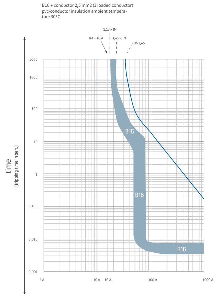
Fig. 14: Characteristic curve for planning example 3
