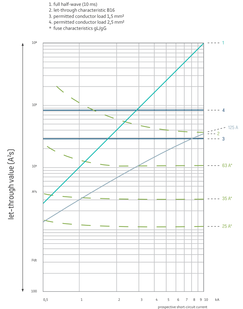
Fig. 16: Let-through energy
