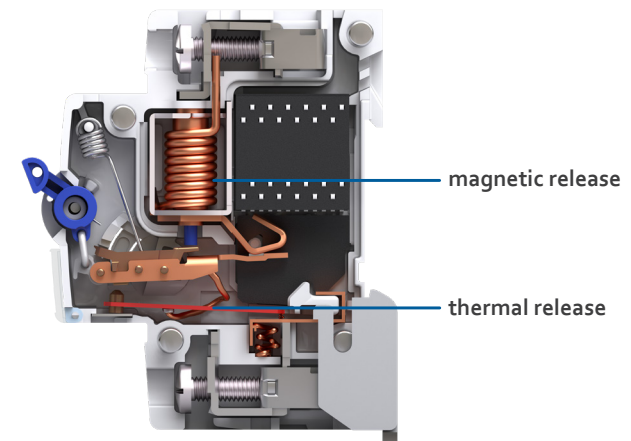
Fig. 2: Overcurrent and short-circuit release
